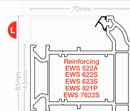
Intermediate transom T EWS 7722
