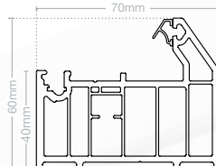
Main frame EWS 7011
