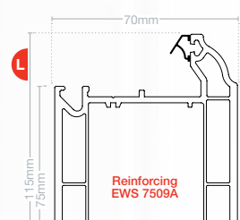
Intermediate transom Z EWS 7723
