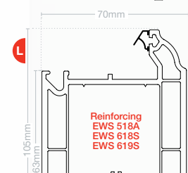
Intermediate transom T EWS 7722
