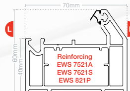
Main frame EWS 7021
