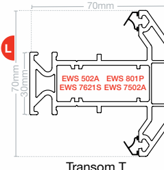
Transom T EWS 7002
