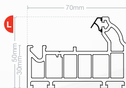
Thermalogik frame EWS 7701 Reinforcing EWS 800P
