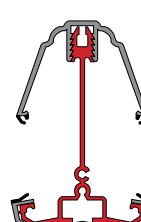
X35VH1 Light Victorian Hip Rafter XRC25 Top Cap XBC1 Bottom Cap
