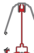
XGH1 Light Georgian Hip Rafter XGC25 Top Cap XBC1 Bottom Cap
