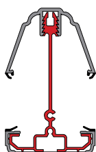
X35T1 Light Transom Rafter XRC25 Top Cap XBC3 Bottom Cap
